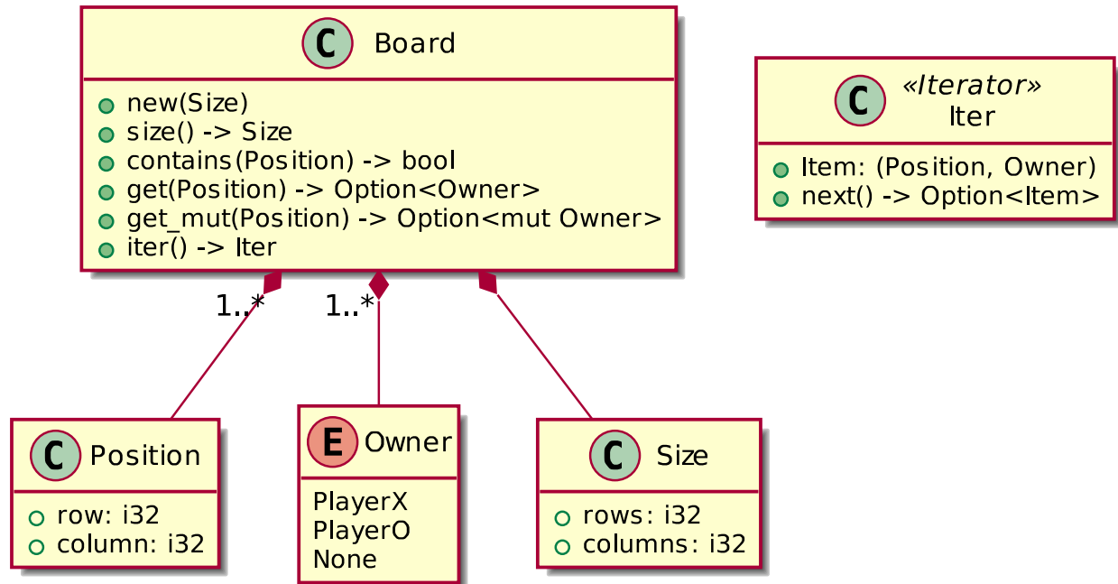
Figure 4.5: The Board structure and supporting types.
