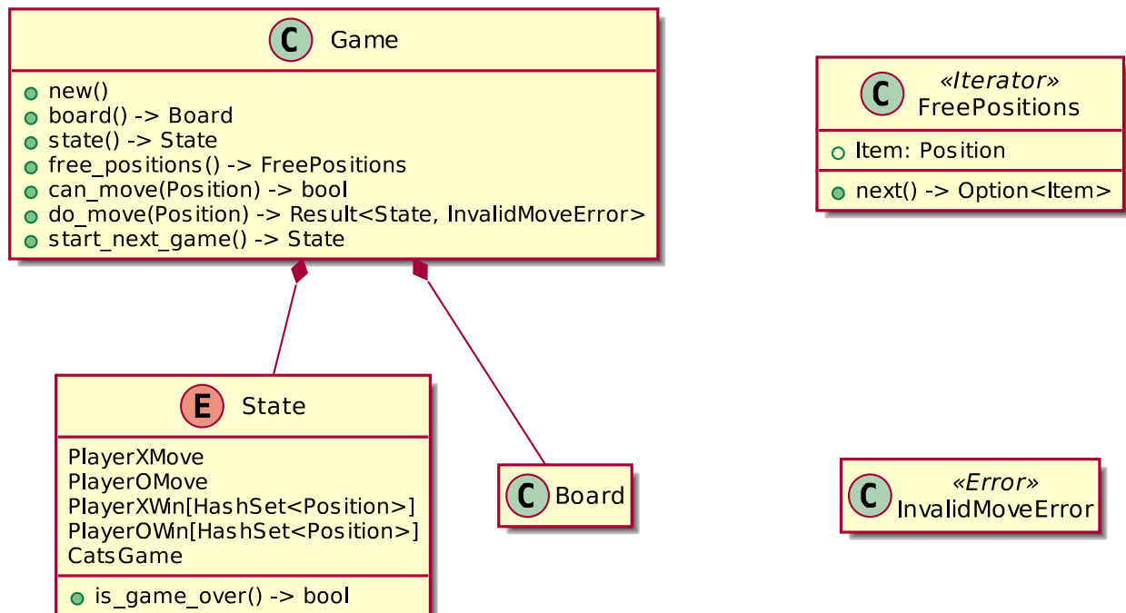
Figure 4.3: The Game structure contains a State and a Board.
