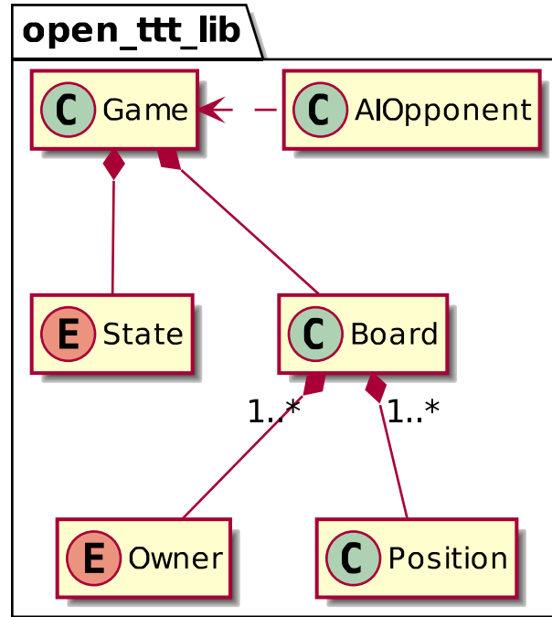
Figure 4.2: Major public modules, structures, and other types. Note: the module contains additional supporting types that are not shown here.
